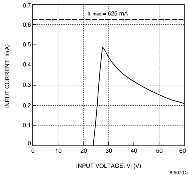
Figure 3. MK010A1, N1 Typical Input Characteristic; I_o = I_{o, \max} ; T_A = 25^\circ\text{C}
