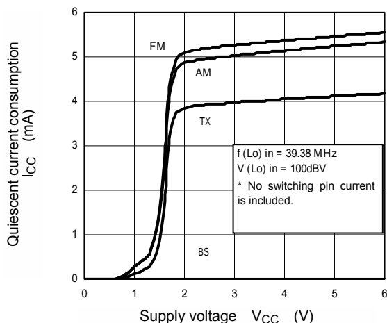
Quiescent Current Consumption – Supply Voltage Characteristics
