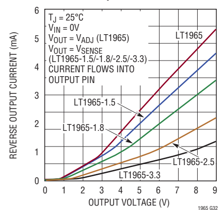
Reverse-Output Current
