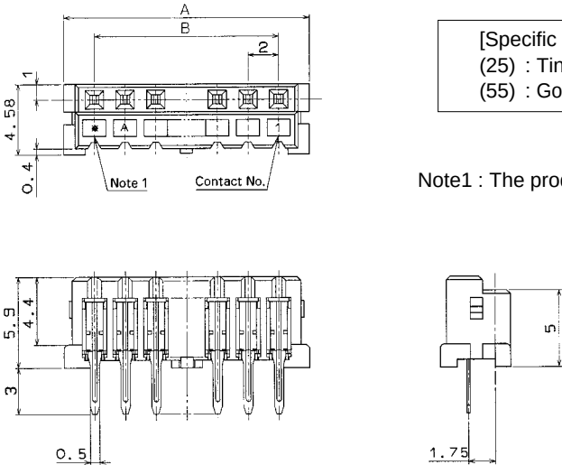
●Board Through-hole Diameter : \phi 0.8^{+0.1}_0
