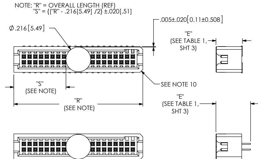
FIG 3 -K: POLYIMIDE FILM PAD
