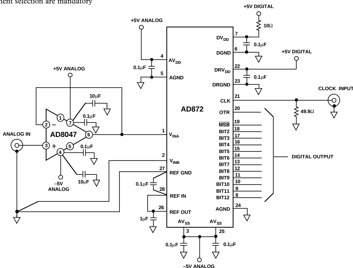
Figure 60. AD8047 Used as Driver for an AD872, a 12-Bit, 10 MSPS A/D Converter
