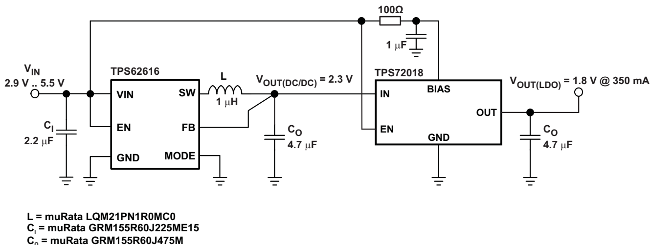
Figure 37. 1.8V Power Rail Featuring Very Low Noise Performance
