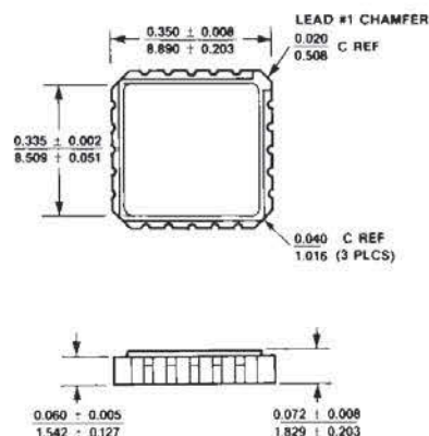
20 Leadless Chip Carrier (LP)
