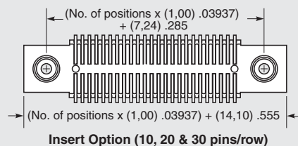
Insert Option (10, 20 & 30 pins/row)
