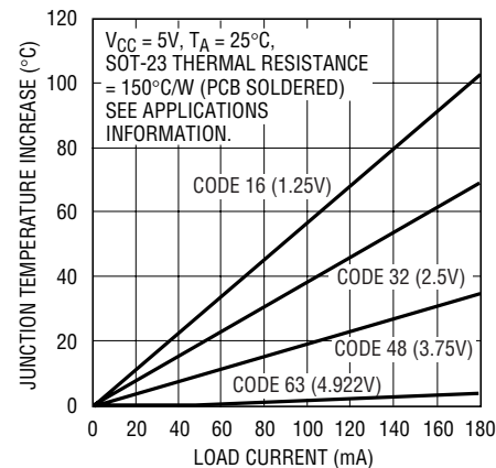
Junction Temperature Increase vs Load Current
