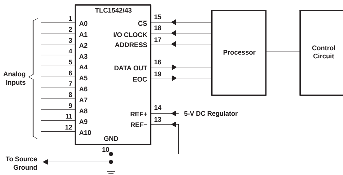
Figure 16. Serial Interface
