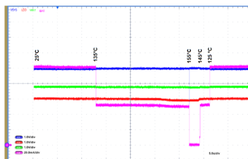
Figure 4. Thermal management
