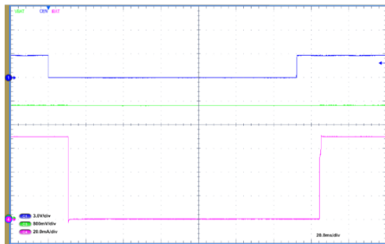
Figure 17. CEN operation
