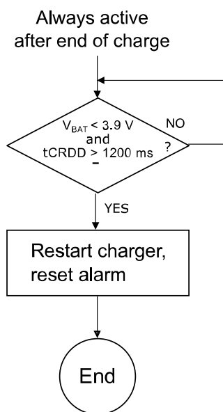
Figure 25. End-of-charge flowchart
