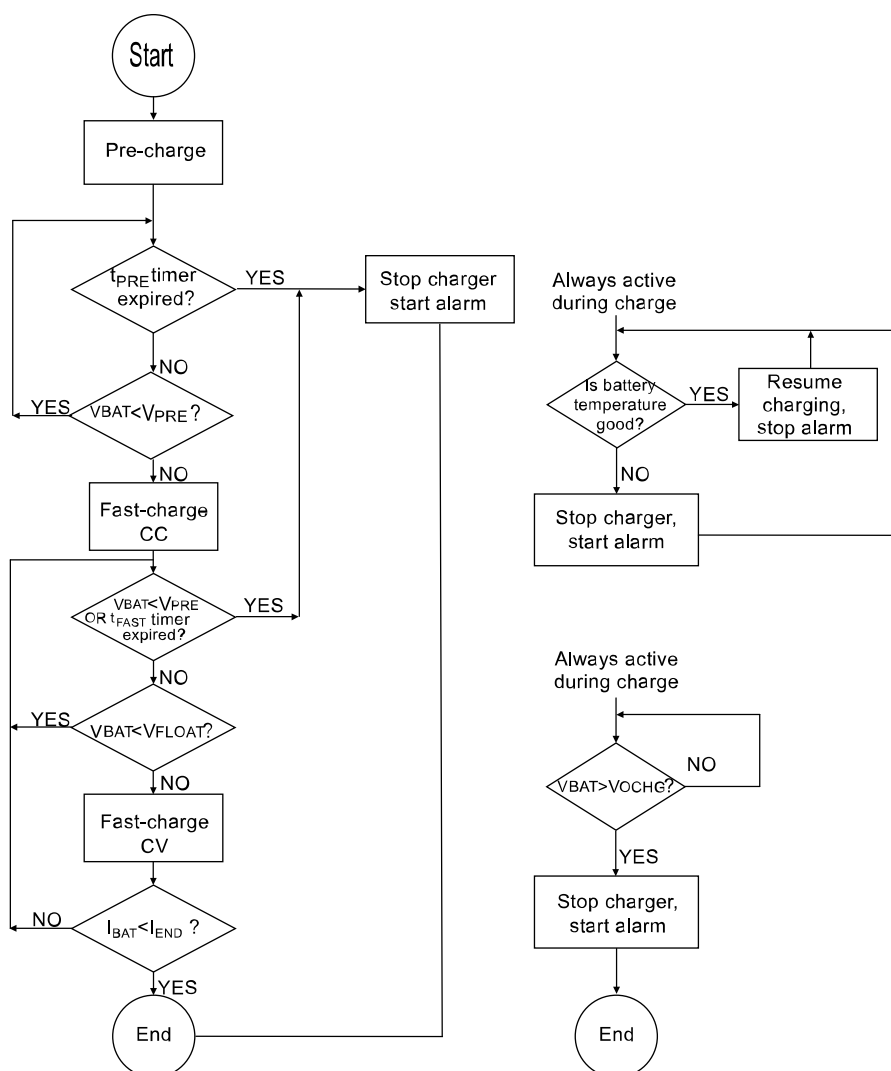
Figure 24. Charging flowchart
