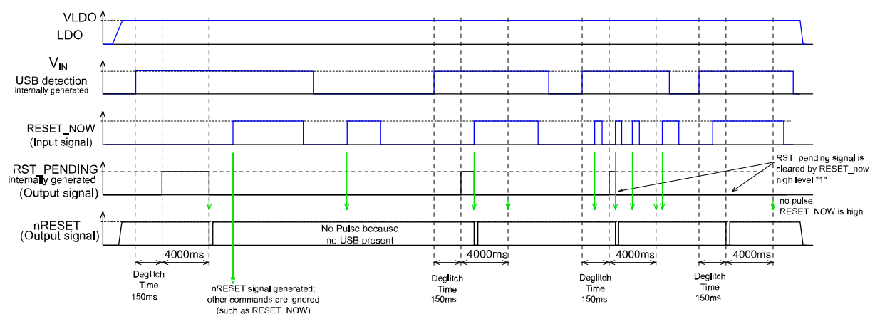
Figure 19. Smart reset timing diagram
