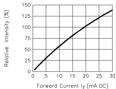
Relative Intensity Vs. Forward Current
