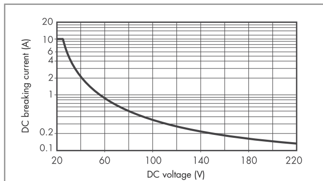
H 36 - Maximum DC1 breaking capacity
