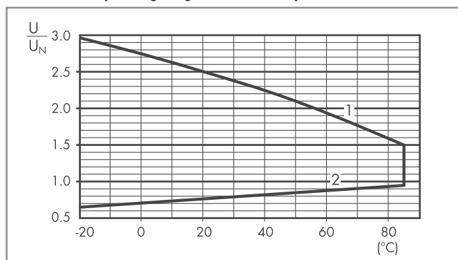
R 36 - DC coil operating range v ambient temperature
