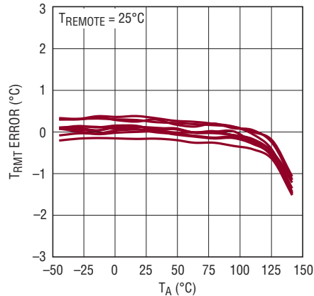
Remote Temperature Error vs Ambient Temperature
