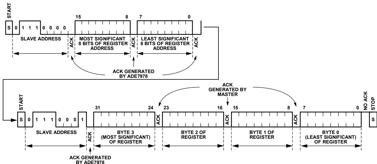
Figure 117. I 2 C Read Operation of a 32-Bit Register
