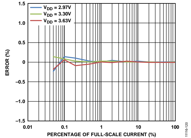
Figure 15. Total Active Energy Error as a Percentage of Reading over Power Supply, PF = 1, T_A = 25^\circ\text{C}
