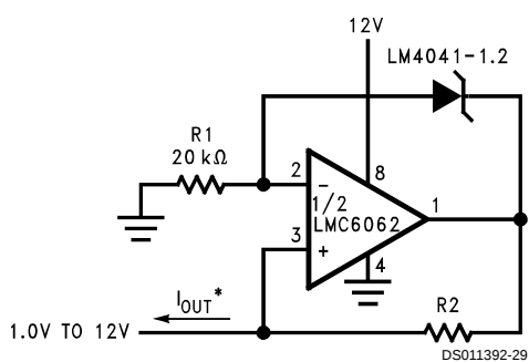
FIGURE 13. Precision 1 \mu A to 1 mA Current Sources
