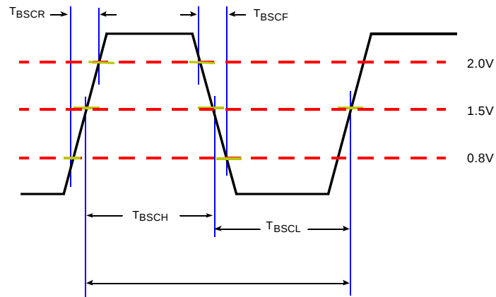
Figure 18. TCK Waveform
