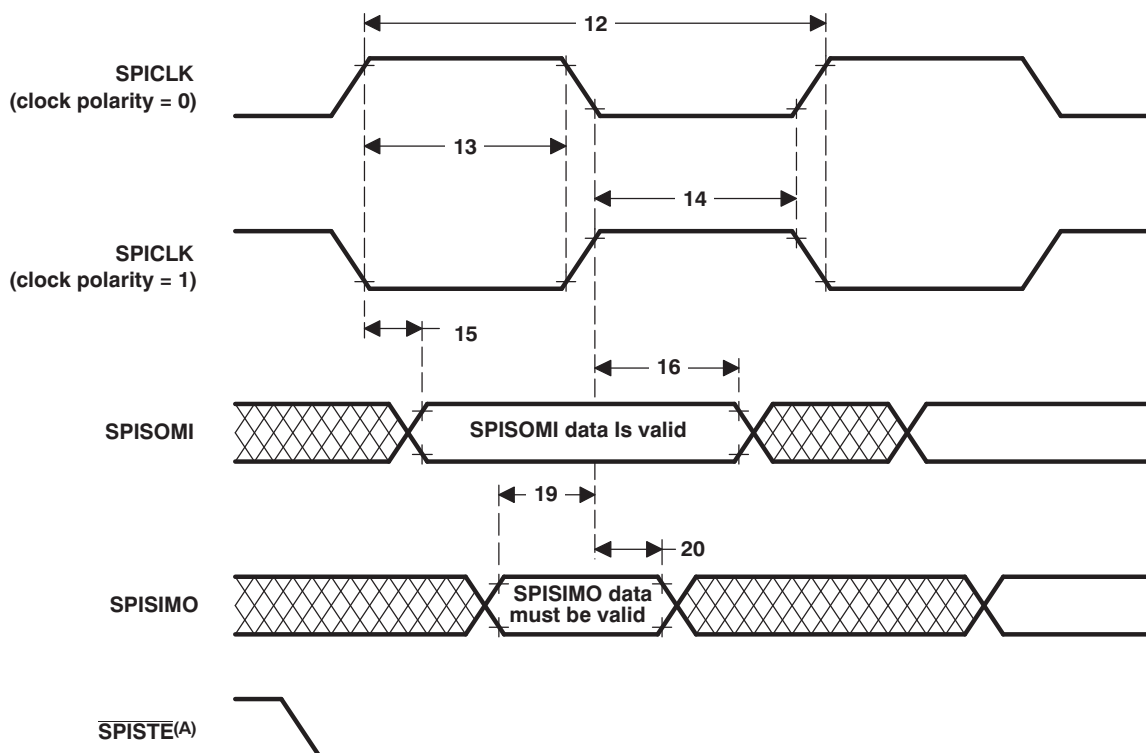
Figure 6-35. SPI Slave Mode External Timing (Clock Phase = 0)
