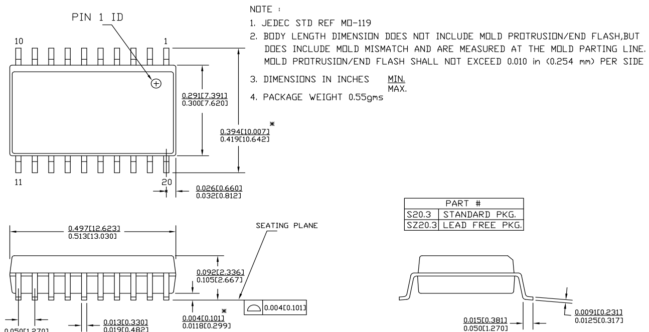
Figure 7. 20-pin SOIC (0.513 × 0.300 × 0.0932 Inches) Package Outline, 51-85024
