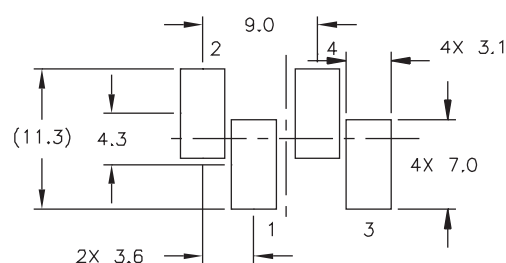
PRIMARY SUGGESTED LAND PATTERN
