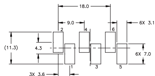
PRIMARY SUGGESTED LAND PATTERN
