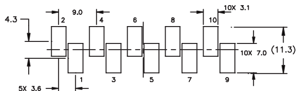
PRIMARY SUGGESTED LAND PATTERN
