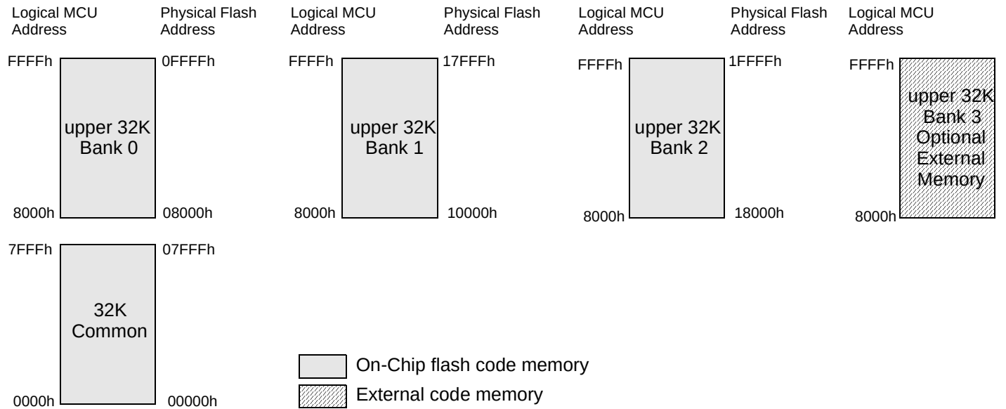
Figure 10. Program/Code Memory Organization EA=1
