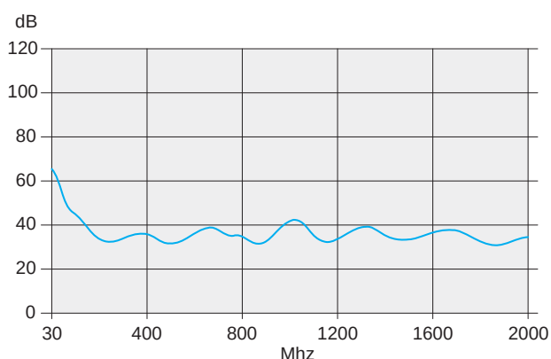
EMC curve
