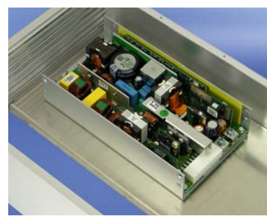
Mounting plate for fitting heavy components
