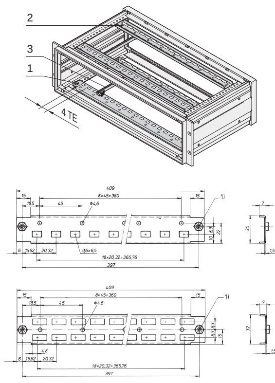
Dimension drawing top: Front support rail, dimension drawing bottom: rear support rail; 1) bush M4, pressed-in
