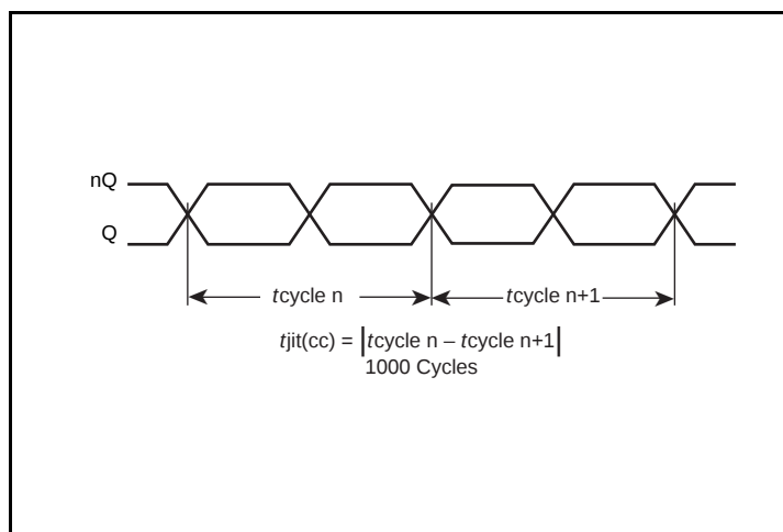
Cycle-to-Cycle Jitter
