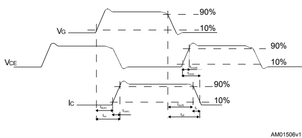
Figure 19. Switching waveform
