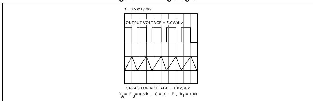
Figure 7. Timing diagram
