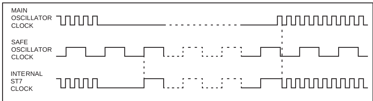
Figure 24. Safe Oscillator Function
