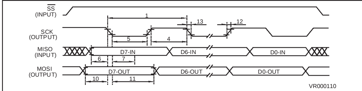
Figure 61. SPI Master Timing Diagram CPHA=1, CPOL=0 1)
