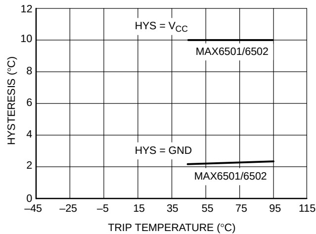
Figure 8. Hysteresis vs. Trip Temperature
