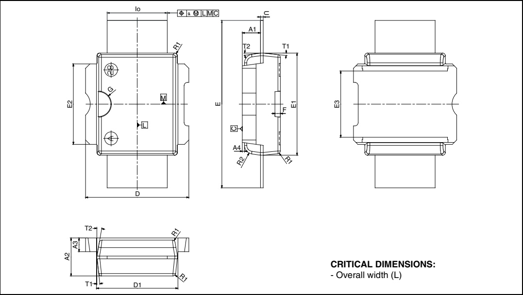
Figure 15. Package dimensions
