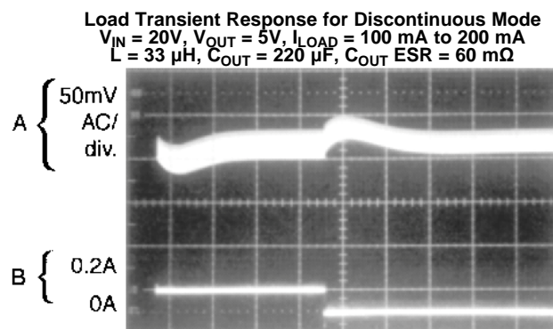
Figure 23. Horizontal Time Base: 2 \mu\text{s} /div.
