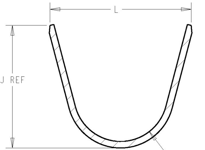
SECTION F-F
