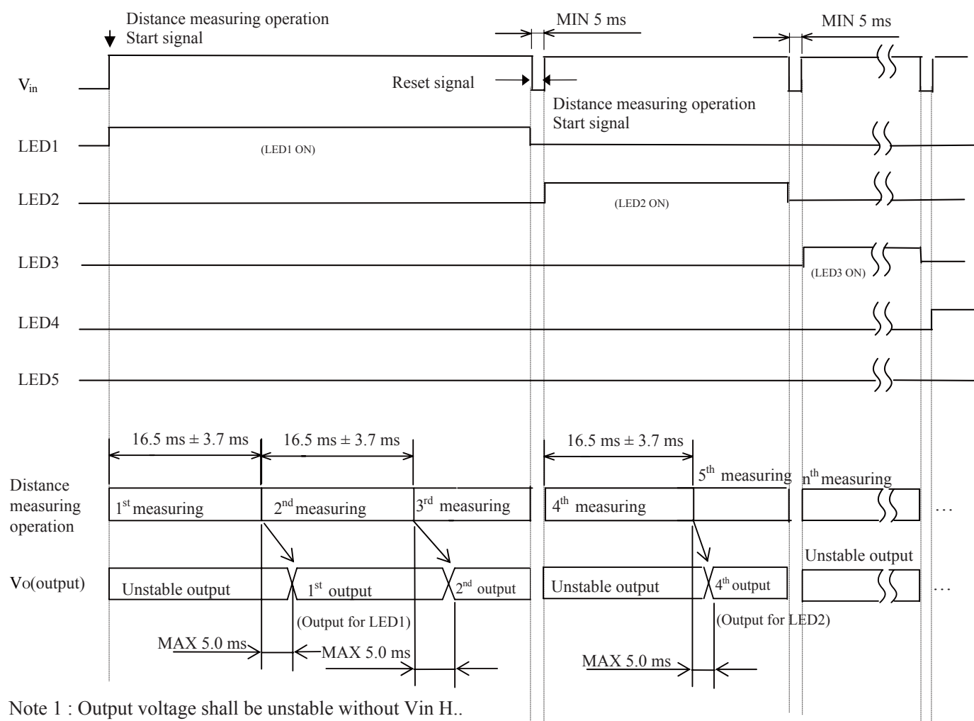
Fig. 1 Timing chart
