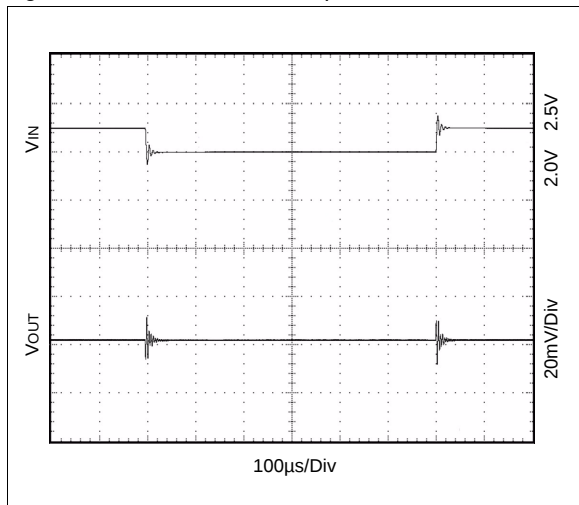
Figure 17. Line Transient Response; I_{OUT} = 350\text{mA}
