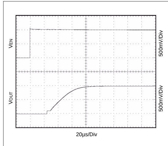
Figure 16. Enable Start-up
