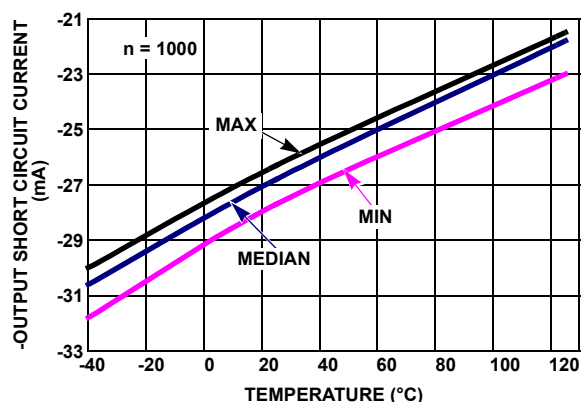
FIGURE 36. -OUTPUT SHORT CIRCUIT CURRENT vs TEMPERATURE V_{IN} = -2.5V , R_L = 10 , V_+ = \pm 2.5V
