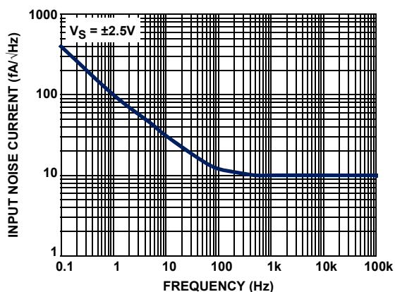
FIGURE 10. CURRENT NOISE vs FREQUENCY
