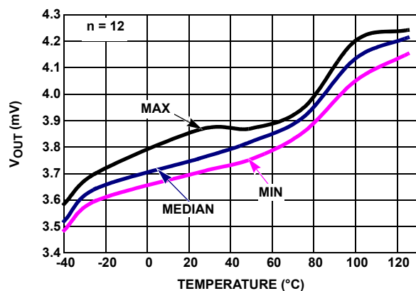
FIGURE 34. V_{OUT} LOW vs TEMPERATURE, V_+ = \pm 2.5V , R_L = 100k
