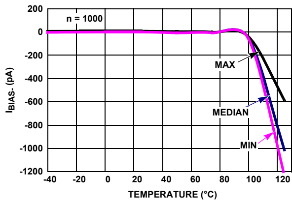
FIGURE 25. I_{BIAS-} vs TEMPERATURE V_+ = 5V , V_- = 0V
