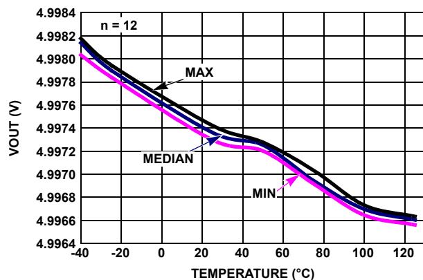
FIGURE 32. V_{OUT} HIGH vs TEMPERATURE, V_+ = \pm 2.5V , R_L = 100k
