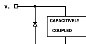
CIRCUIT 4
