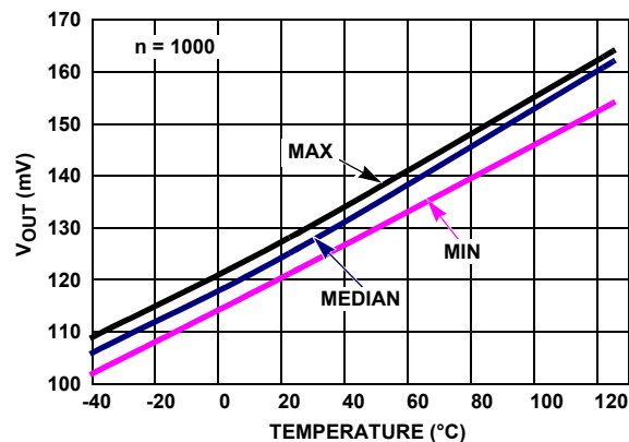
FIGURE 33. V_{OUT} LOW vs TEMPERATURE, V_+ = \pm 2.5V , R_L = 1k
