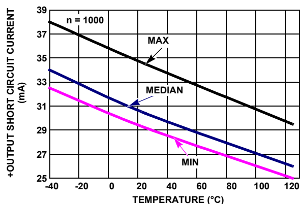
FIGURE 35. +OUTPUT SHORT CIRCUIT CURRENT vs TEMPERATURE V_{IN} = +2.5V , R_L = 10 , V_+ = \pm 2.5V
