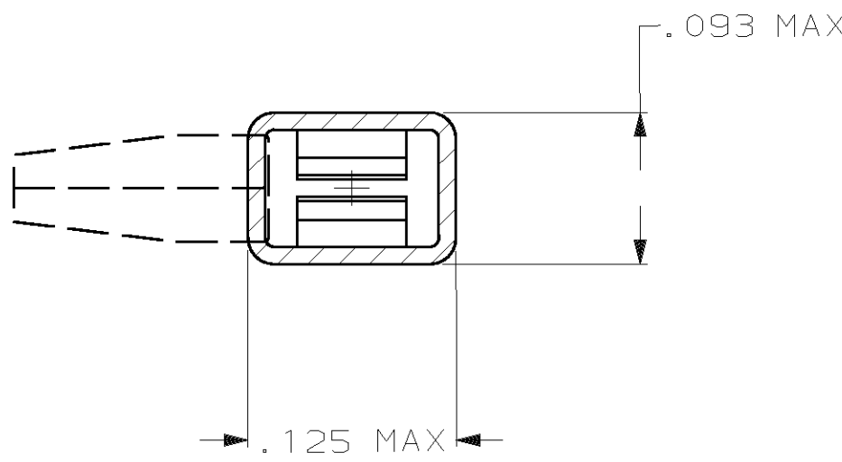
SECTION Y-Y
