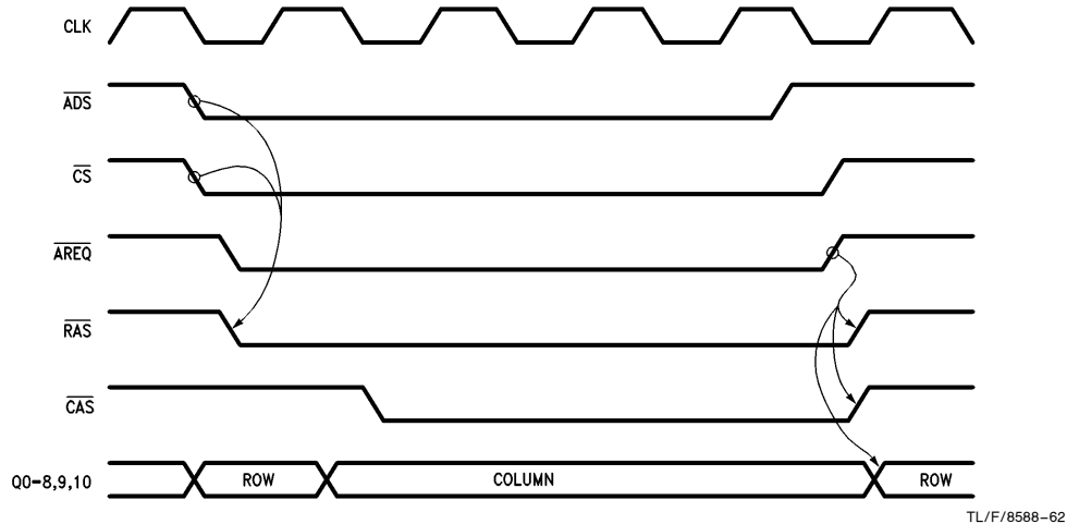
FIGURE 8b. Access Mode 1
