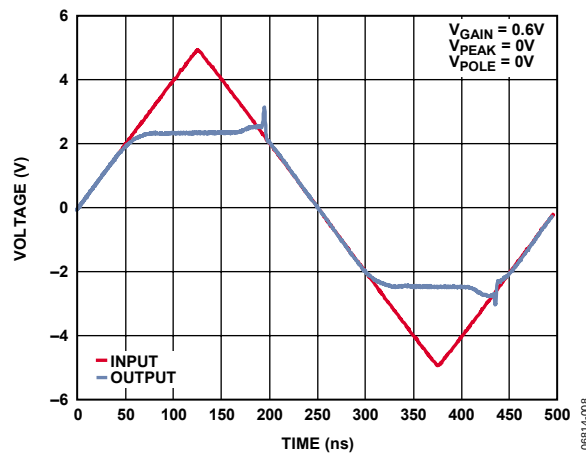
Figure 10. Overdrive Recovery
