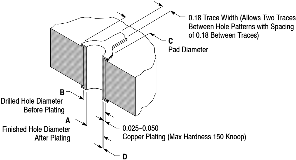
PC Board Contact Hole Dimensions
