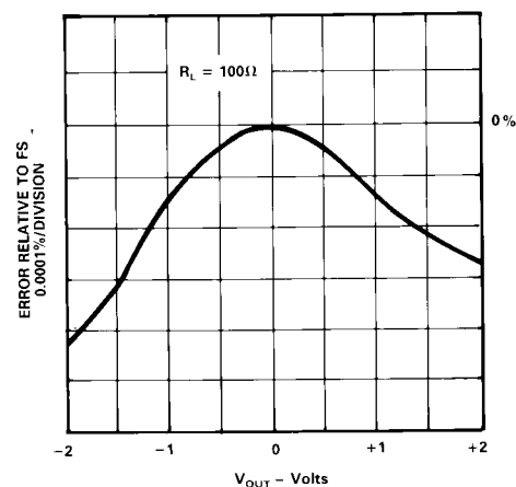
DC Nonlinearity vs. V_{OUT}
