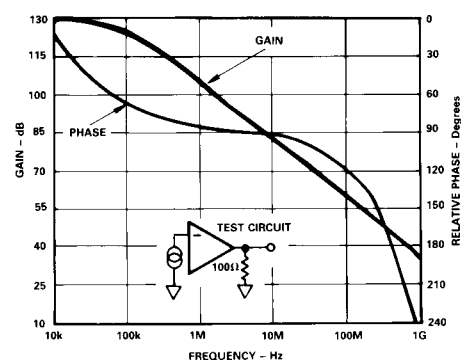
Open Loop Transimpedance Gain [T(s) \text{ Relative to } 1\text{ }\Omega]
