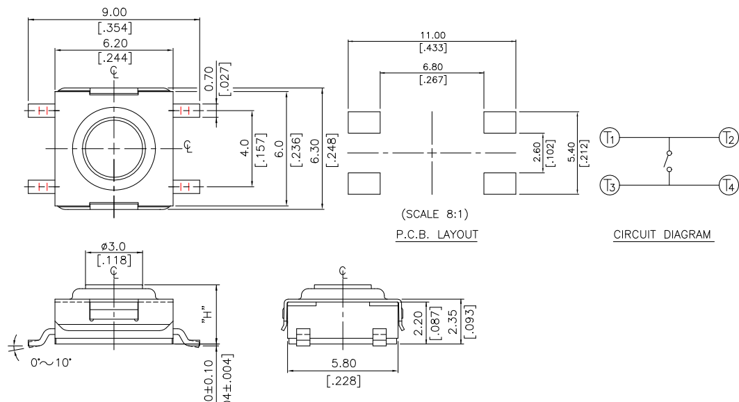
Model SWTW-G (Top Actuation, SMD G pin style, 6 x 6 mm)
