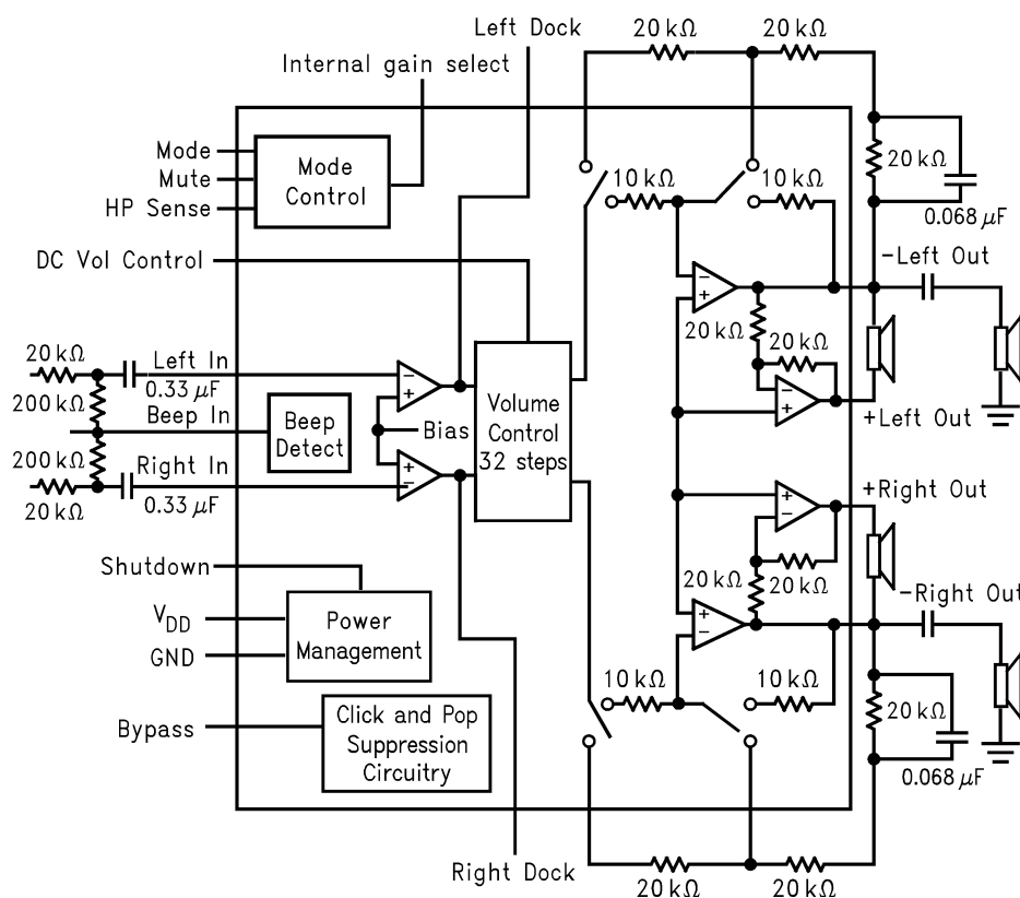
Figure 1. LM4938 Block Diagram
