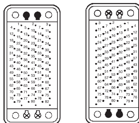
Plug Receptacle
