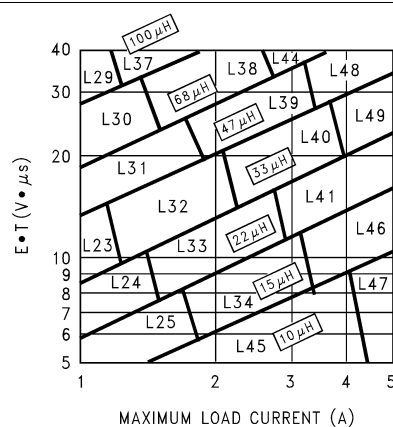
Figure 7-5. LM2678-Adjustable
