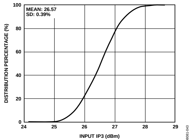
Figure 28. Input IP3 Distribution
