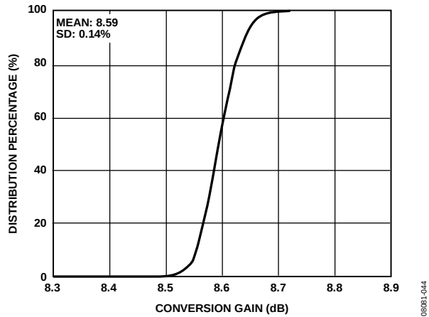
Figure 27. Power Conversion Gain Distribution
