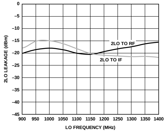
Figure 37. 2LO Leakage vs. LO Frequency
