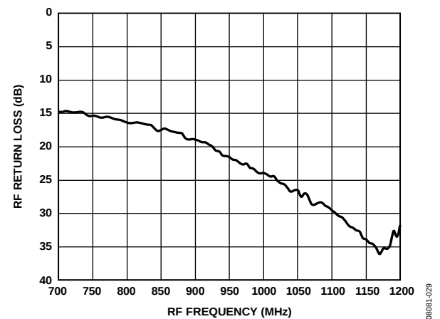
Figure 31. RF Port Return Loss, Fixed IF
