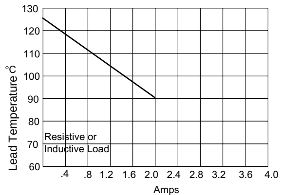
Figure 4 Forward Current Derating
