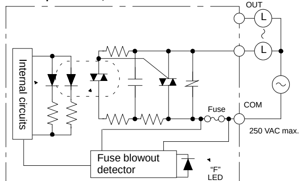
Triac Output: OA223, OA224
