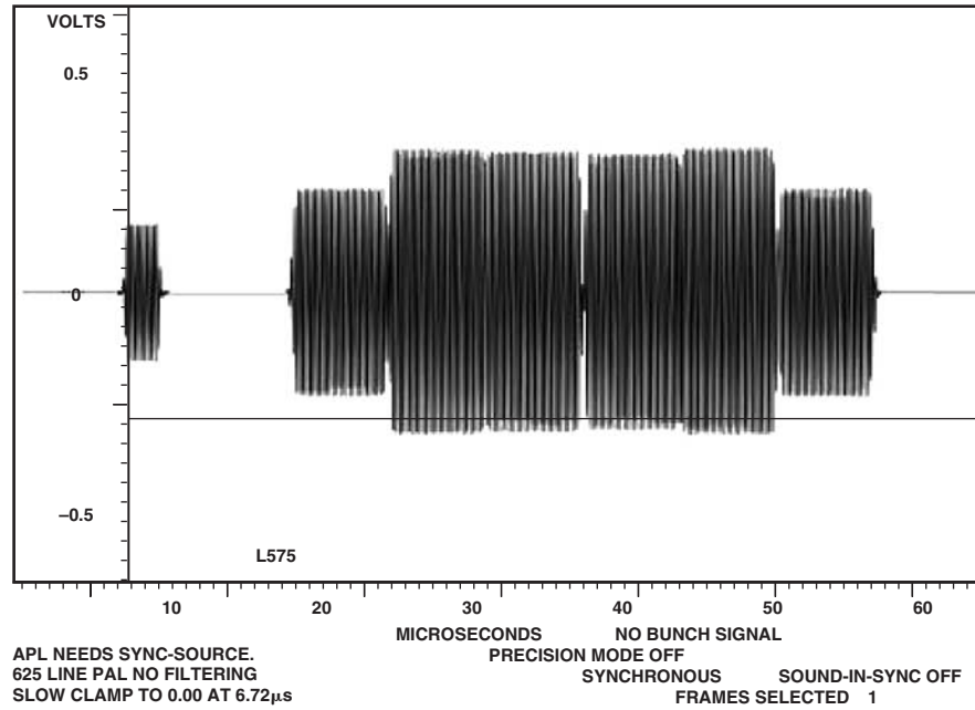
Figure 110. PAL Chroma
