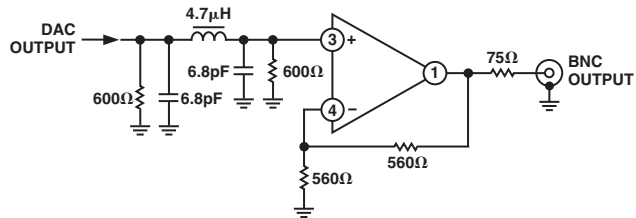
Figure 57. Example of Output Filter for PS, 8× Oversampling
