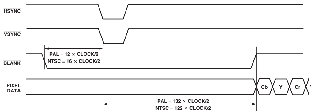
Figure 87. SD Timing Mode 2 Even to Odd Field Transition Master/Slave
