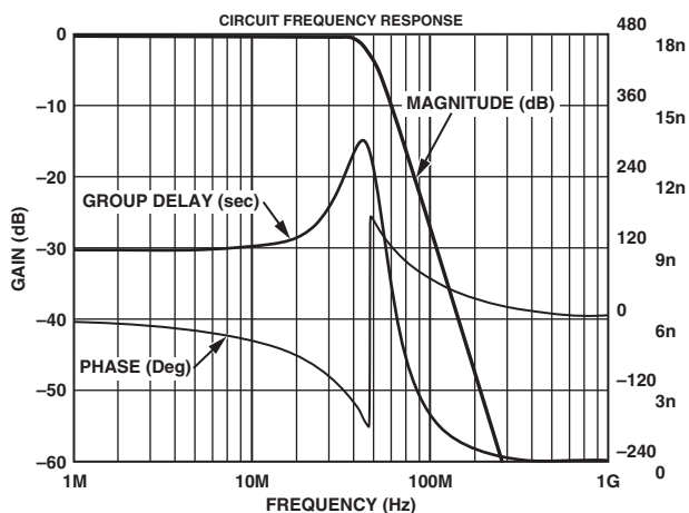
Figure 60. Filter Plot for Output Filter for HDTV, 2× Oversampling
