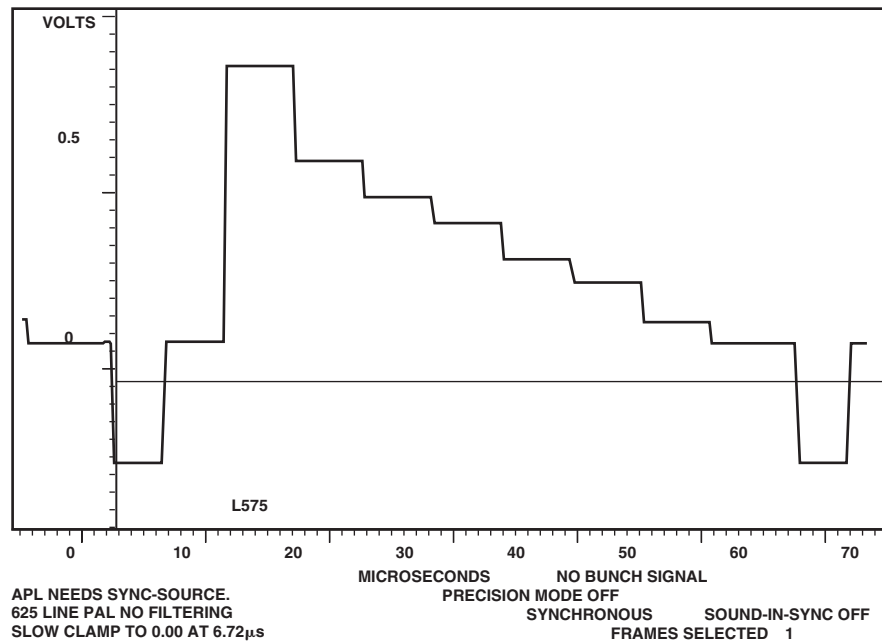
Figure 111. PAL Luma
