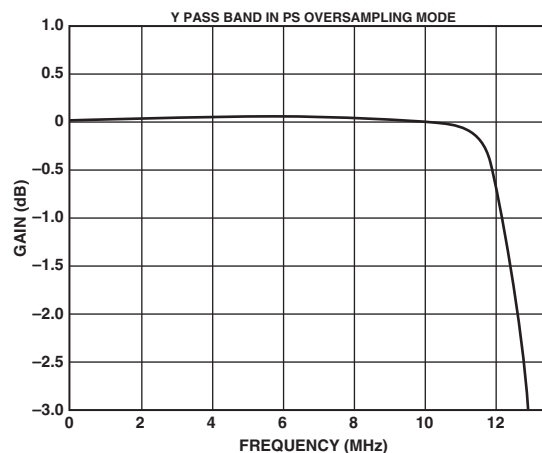
TPC 4. PS—Y 8× Oversampling Filter (Pass Band)
