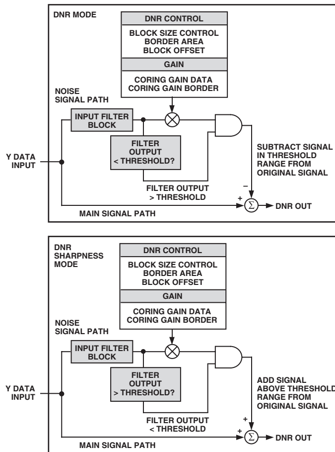
Figure 48. DNR Block Diagram
