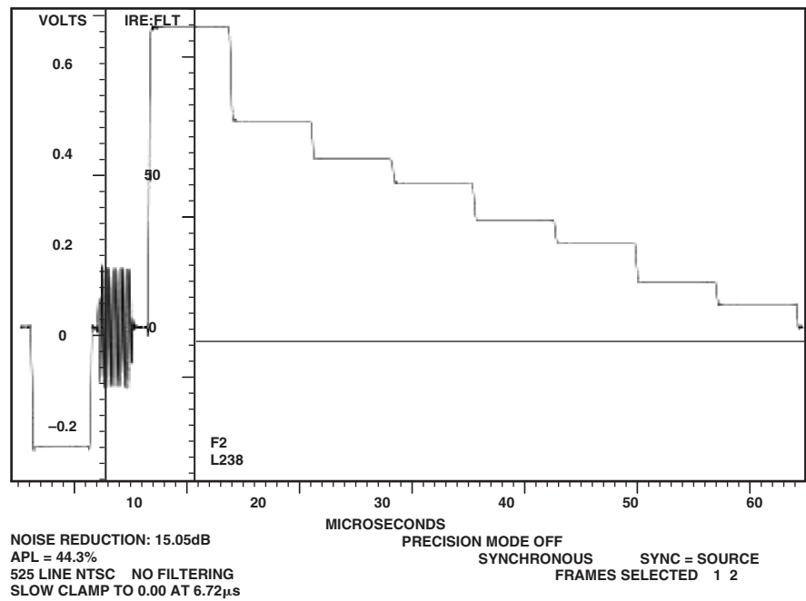
Figure 108. NTSC Luma
