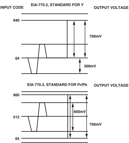
Figure 94. EIA 770.3 Standard Output Signals (1080i, 720p)
