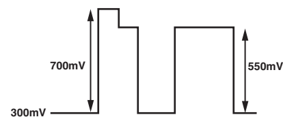
Figure 98. SD RGB Output Levels—RGB Sync Disabled
