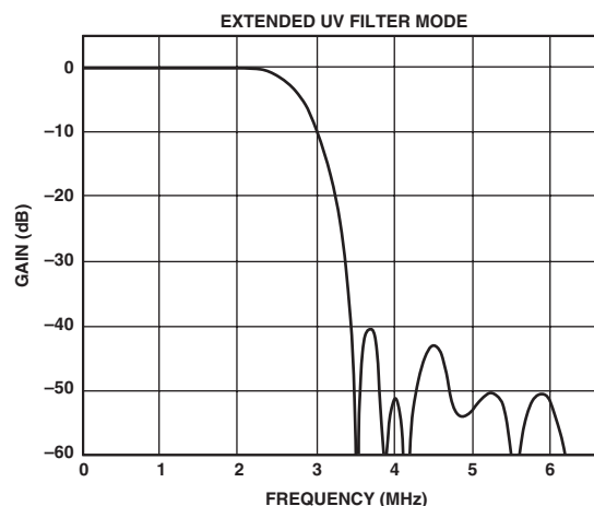
Figure 38. UV SSAF Filter
