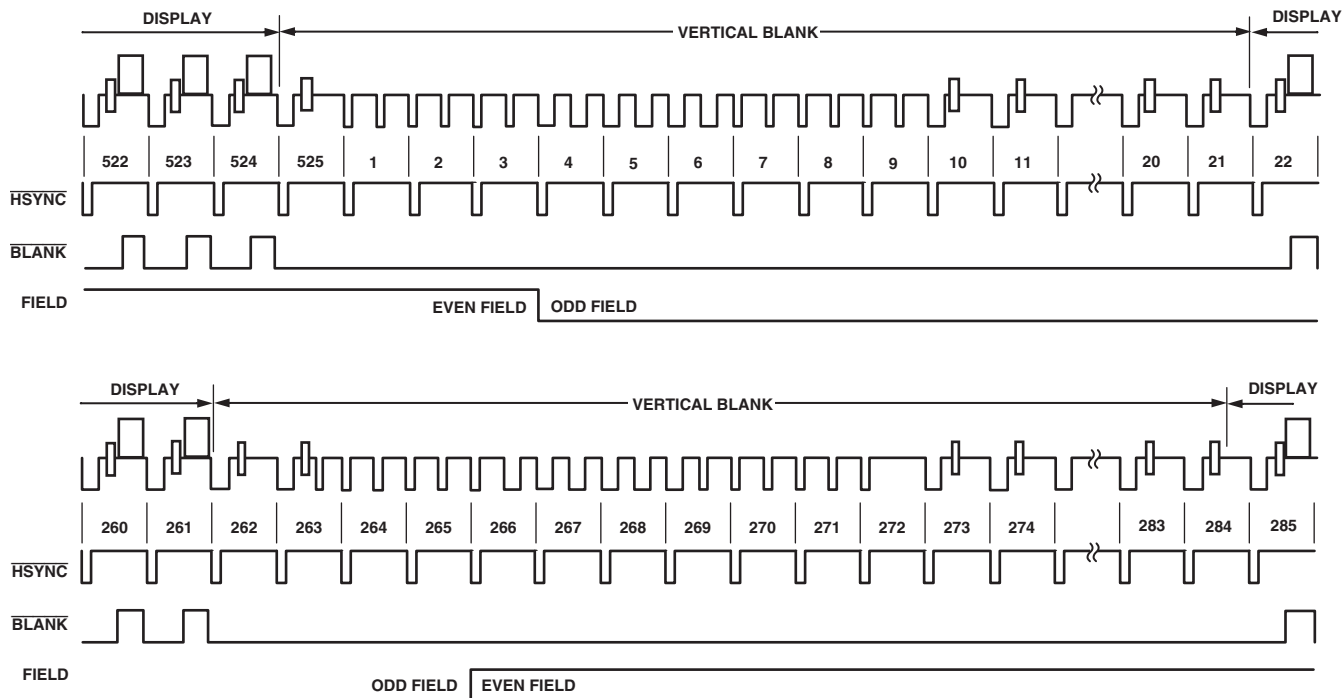
Figure 82. SD Slave Mode 1 (NTSC)
