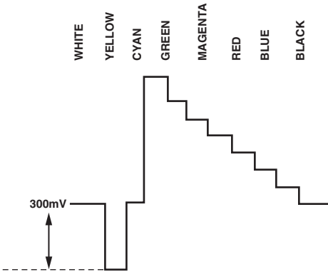
Figure 105. Y Levels—PAL
