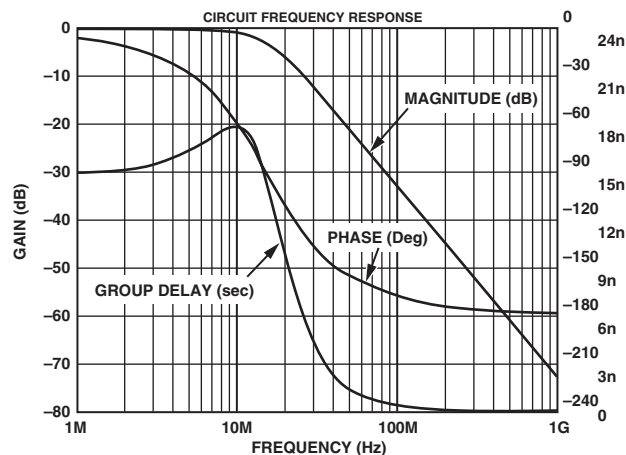
Figure 56. Filter Plot for Output Filter for SD, 16× Oversampling
