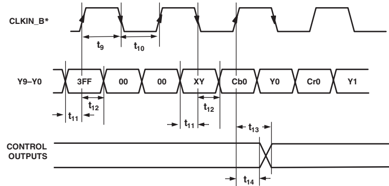
Figure 5. PS 4:2:2 1 × 10-Bit Interleaved at 54 MHz \overline{HSYNC}/\overline{VSYNC} Input Mode [Input Mode 111]
