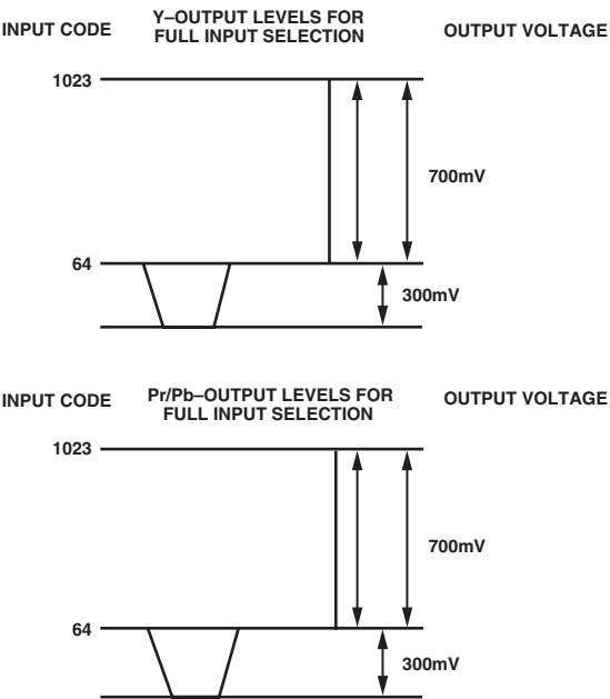
Figure 95. Output Levels for Full Input Selection
