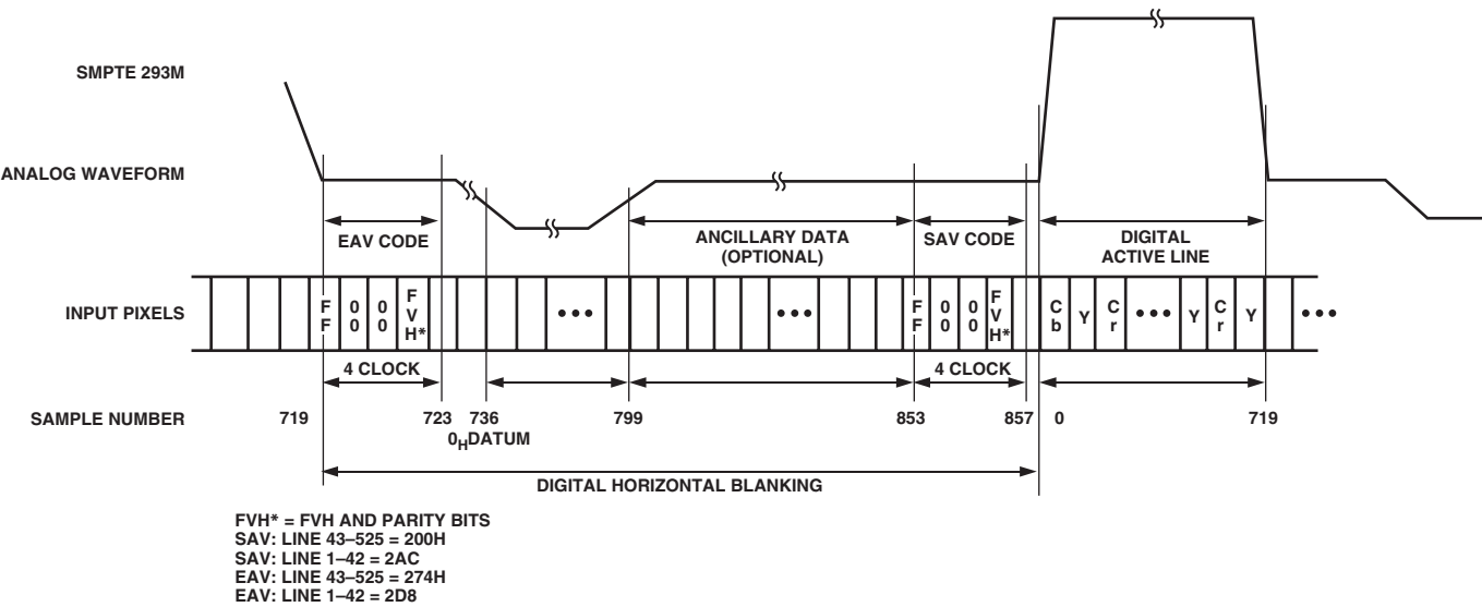
Figure 113. EAV/SAV Input Data Timing Diagram—SMPTE 293M
