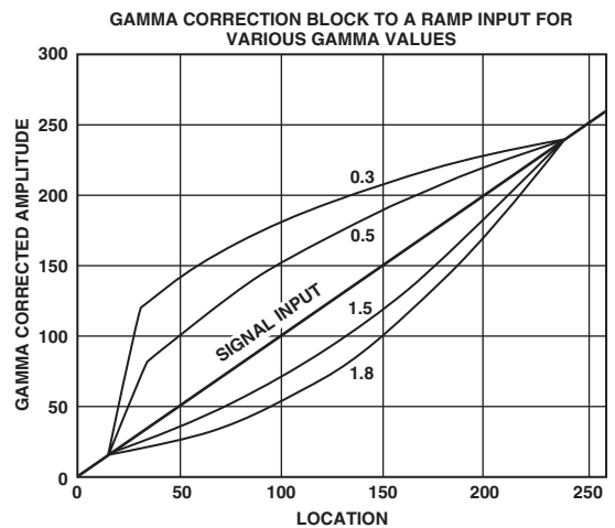
Figure 42. Signal Input (Ramp) and Selectable Output Curves
