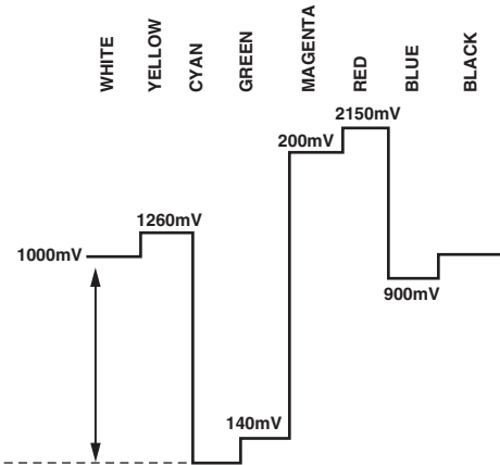
Figure 103. U Levels—PAL
