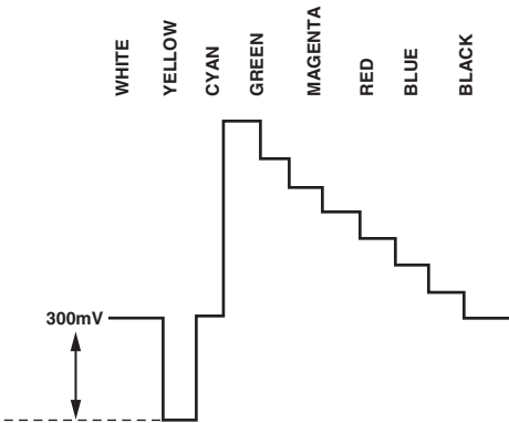
Figure 104. Y Levels—NTSC
