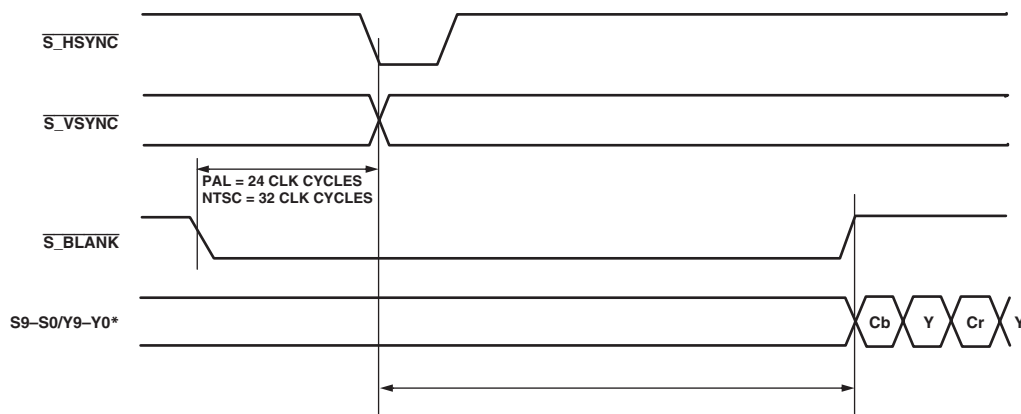
Figure 15. SD Timing Input for Timing Mode 1
