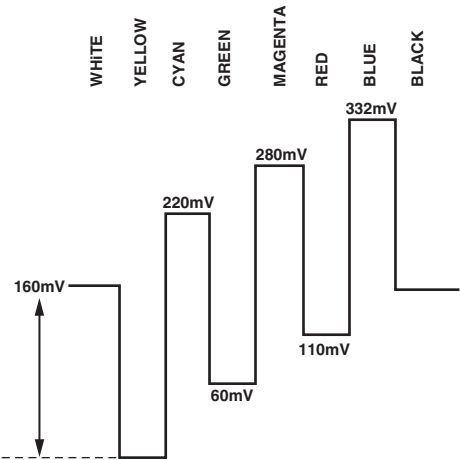
Figure 100. U Levels—NTSC
