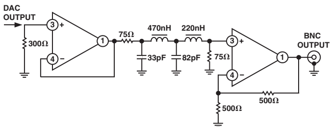
Figure 58. Example of Output Filter for HDTV, 2× Oversampling
