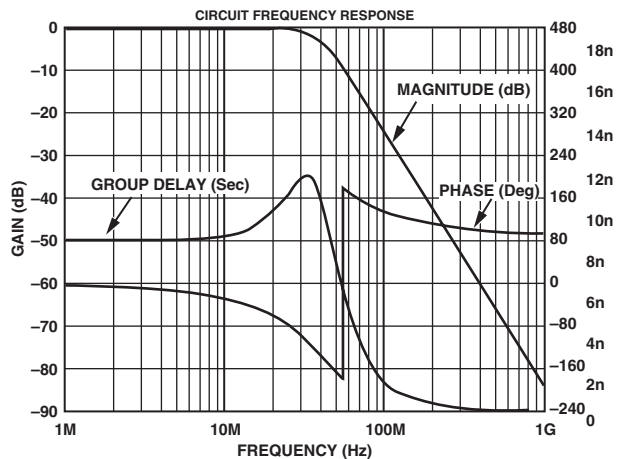
Figure 59. Filter Plot for Output Filter for PS, 8× Oversampling
