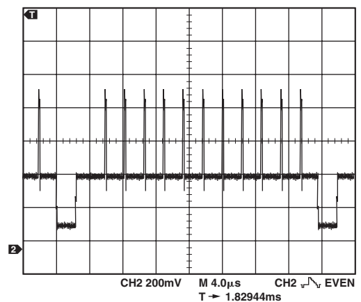
Figure 72. 525p Hatch Pattern
