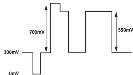
Figure 99. SD RGB Output Levels—RGB Sync Enabled
