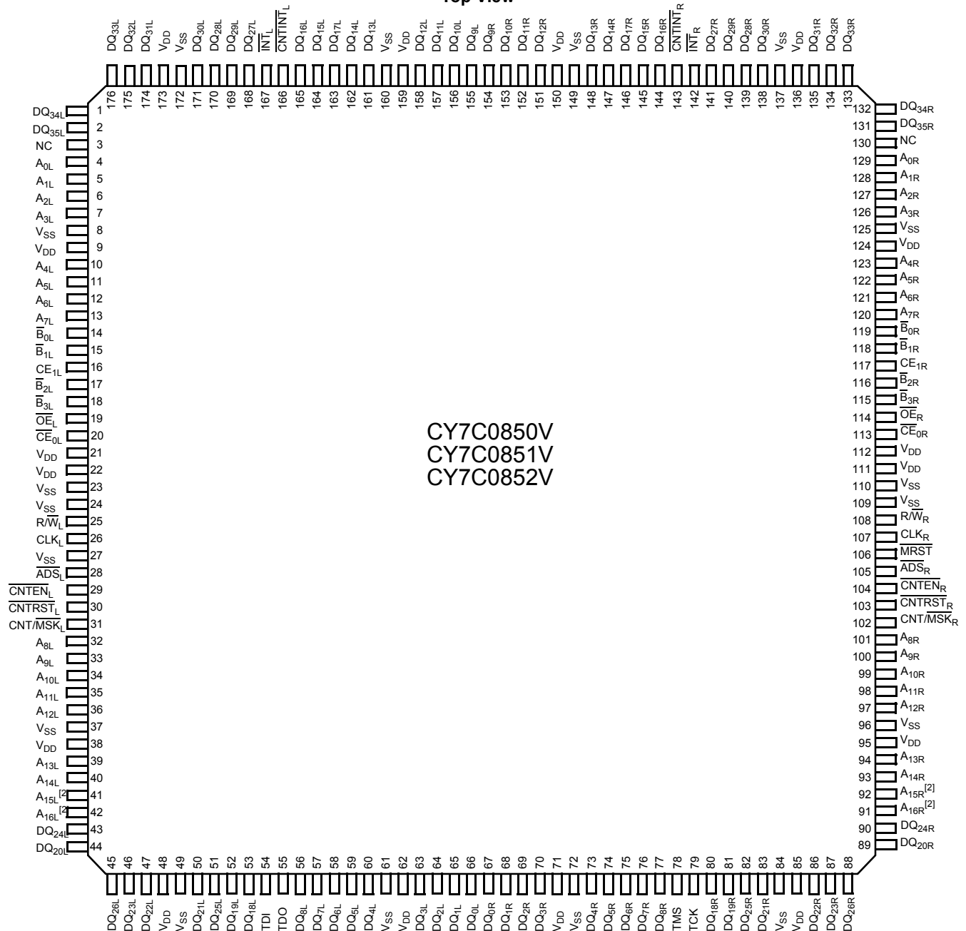
176-pin Thin Quad Flat Pack (TQFP) Top View
