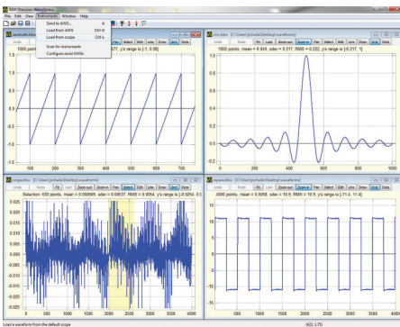
WaveXpress software
