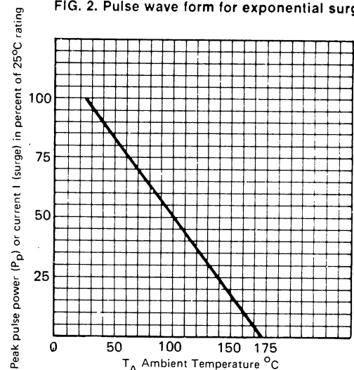
FIG. 3. Derating curve
